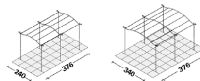
extension L 186
